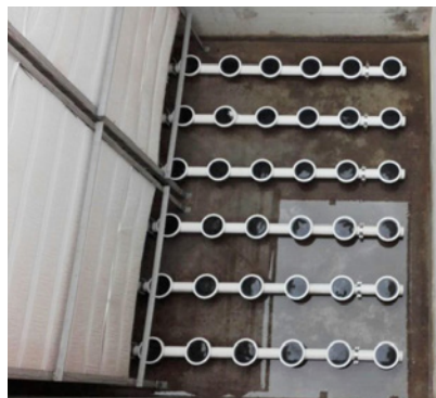
Quantaer Fine Bubble Aeration System
