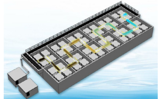
Nebula Flow Pattern
